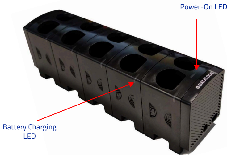
MC-P096-M2 UNIT + 4 MC-P096-E2 UNITS Maximum allowed configuration (4 extension units = 10 batteries)
