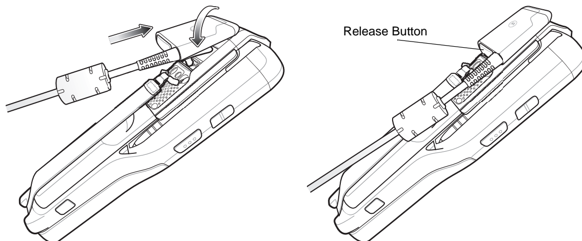
Figure 8-16 Cable Installation
