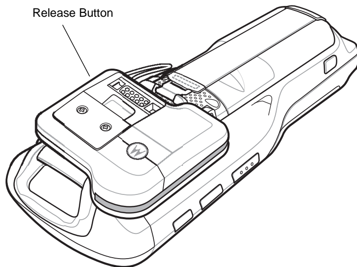
Figure 8-11 MSR Installation
