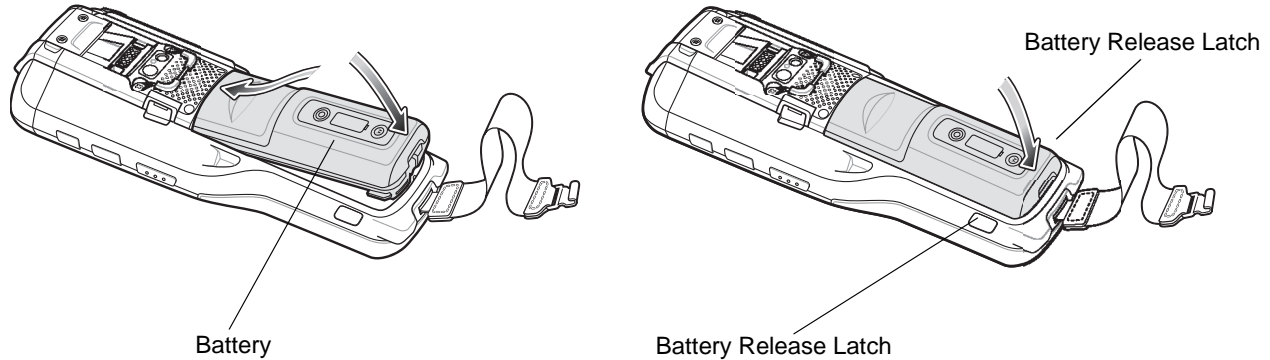
Figure 1-8 Inserting the Battery
