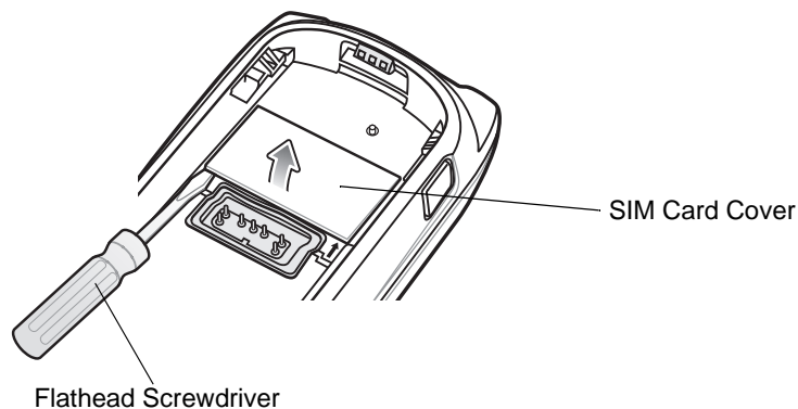
Figure 1-5 SIM Card Cover Removal
