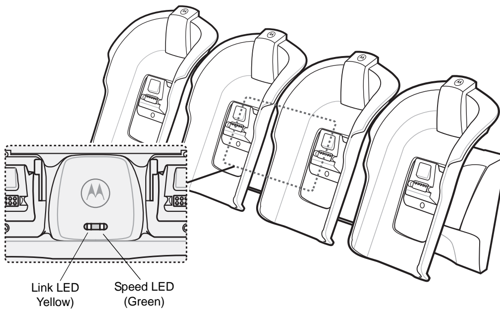
Figure 8-7 Four Slot Ethernet Cradle LED Indications
