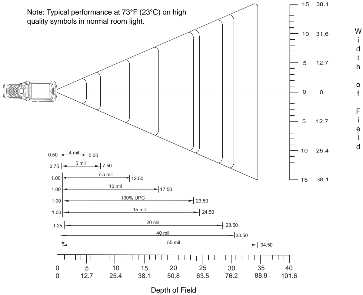
Figure 4-4 MC9500-K Laser Scanner 47° Decode Zone
