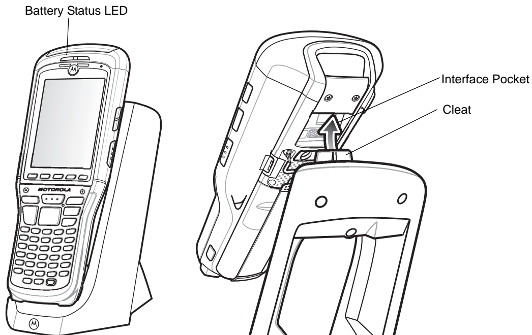
Figure 8-2 MC9500-K Battery Charging
