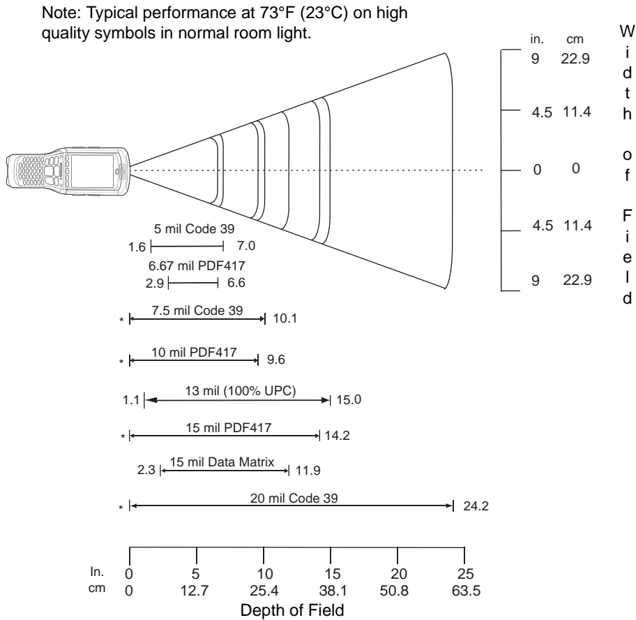
Figure 4-8 MC9500-K Imager Decode Ranges
