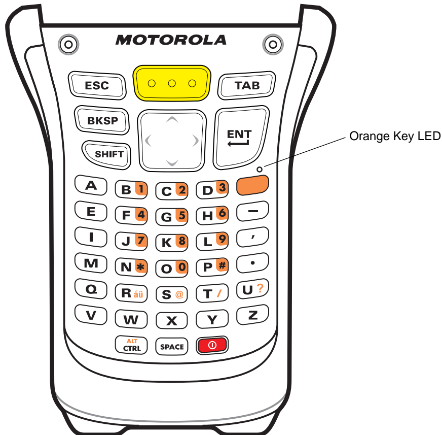
Figure C-1 Alpha Primary Keypad Configuration
