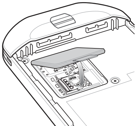
Figure 1-13 Replace Access Door
