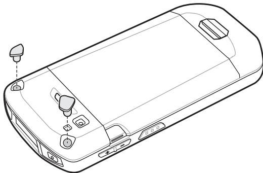
Figure 6-25 Remove Plugs
