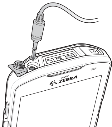
Figure 6-33 Audio Adapter Installation
