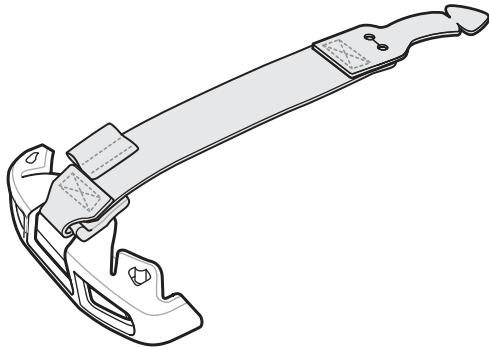
Figure 6-24 Basic Hand Strap Kit
