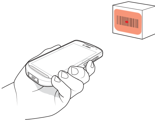
Figure 4-2 Imager Scanning
