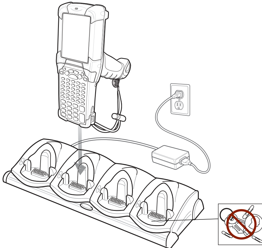
Figure 7-4 Four Slot Charge Only Cradle
