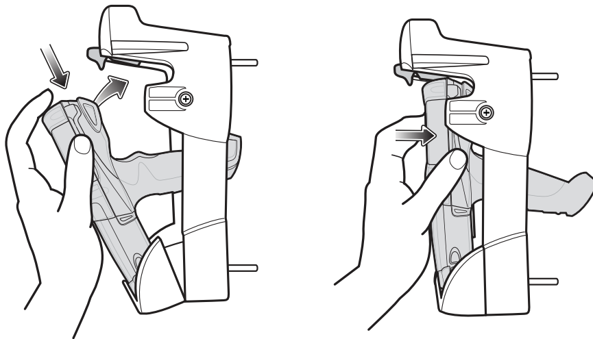
Figure 7-13 Insert MC92N0-G into Forklift Cradle
