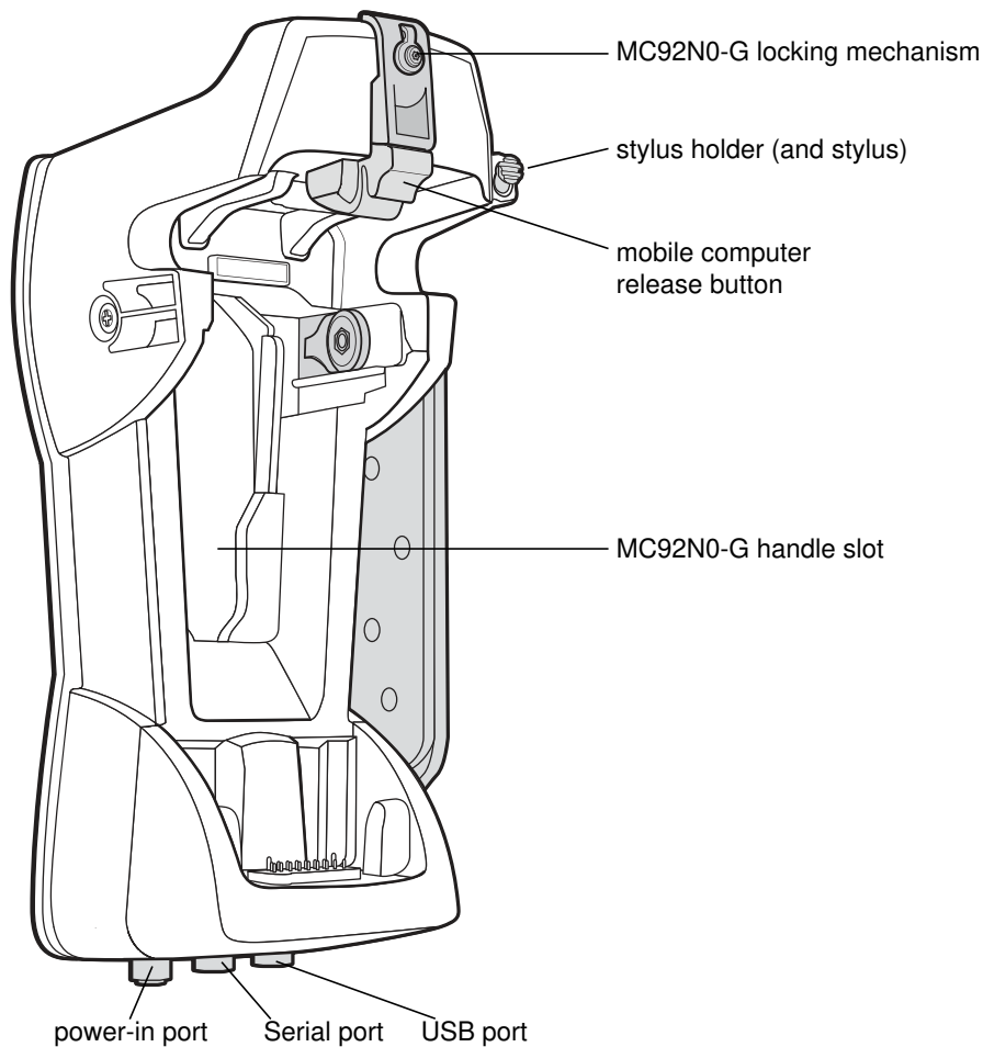
Figure 7-12 Forklift Cradle
