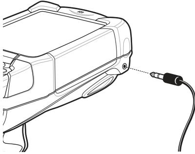
Figure 2-24 Using a Headset (MC92N0-G Shown)
