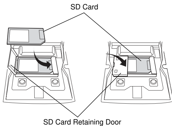
Figure 7-1 Inserting the SD Card
