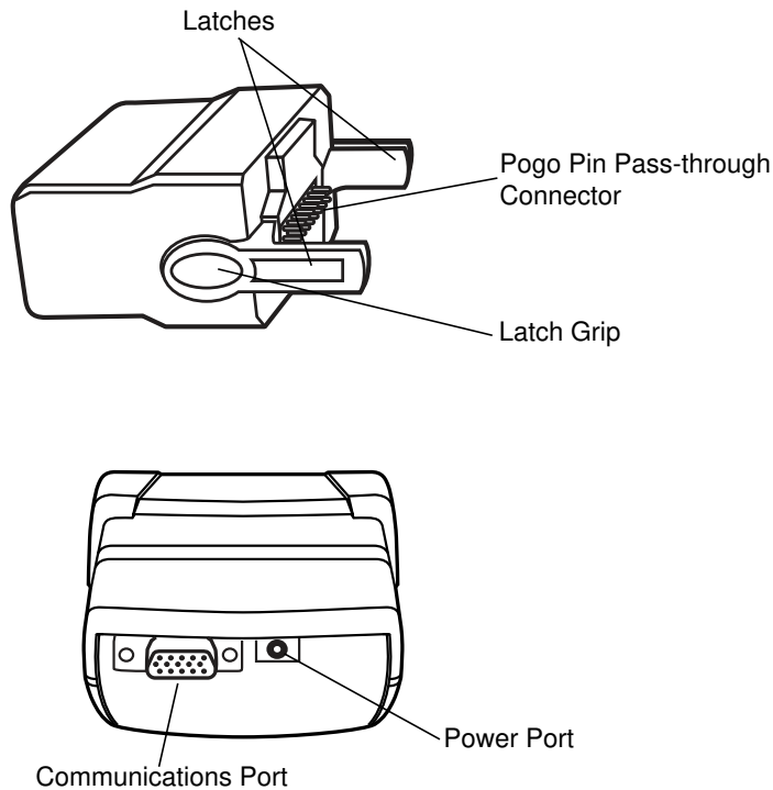
Figure 7-6 Cable Adapter Module
