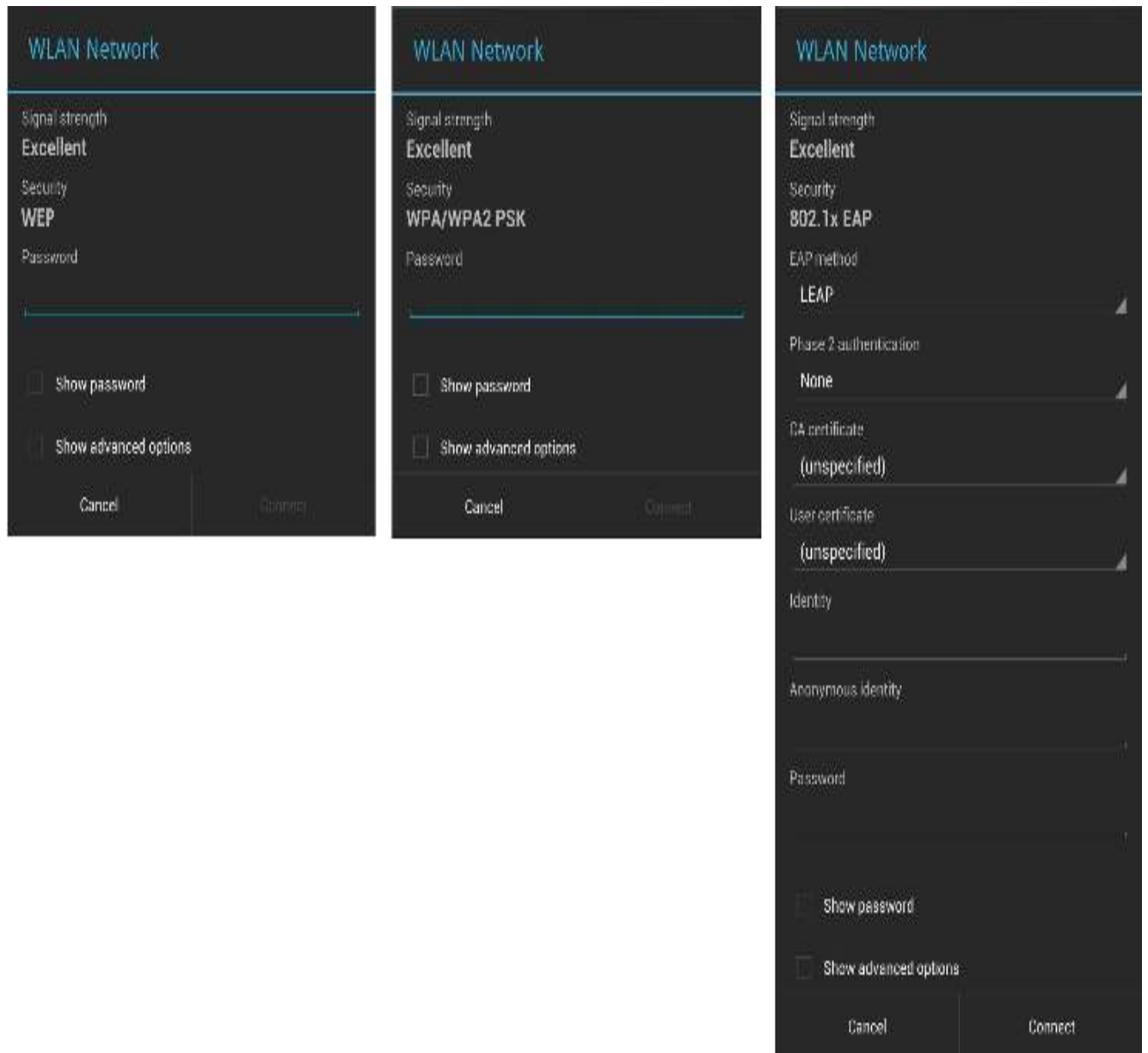
Figure 3-33 WLAN Network Security Dialog Box
