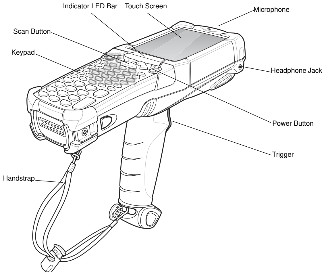
Figure 1-1 MC92N0-G
