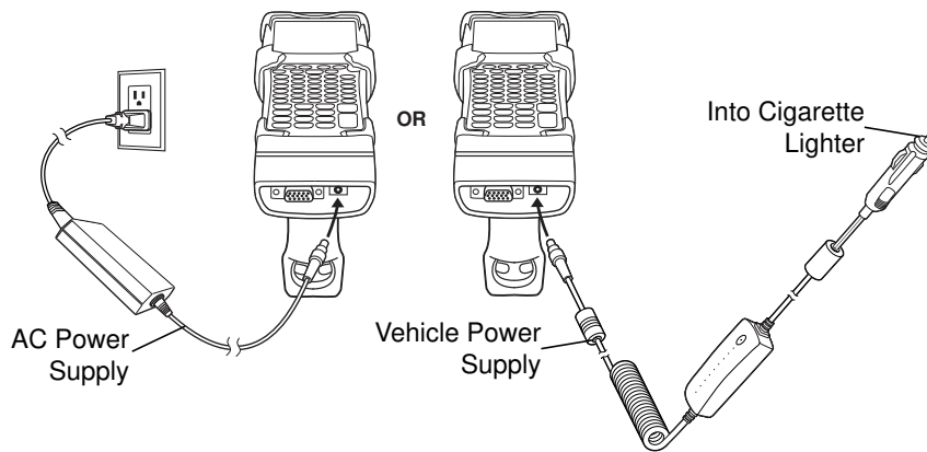
Figure 7-8 CAM Power Connection
