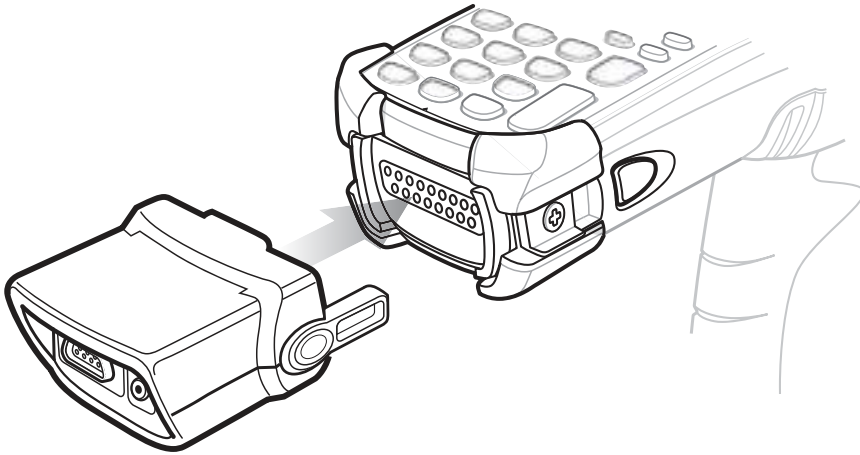
Figure 7-7 Attaching the CAM
