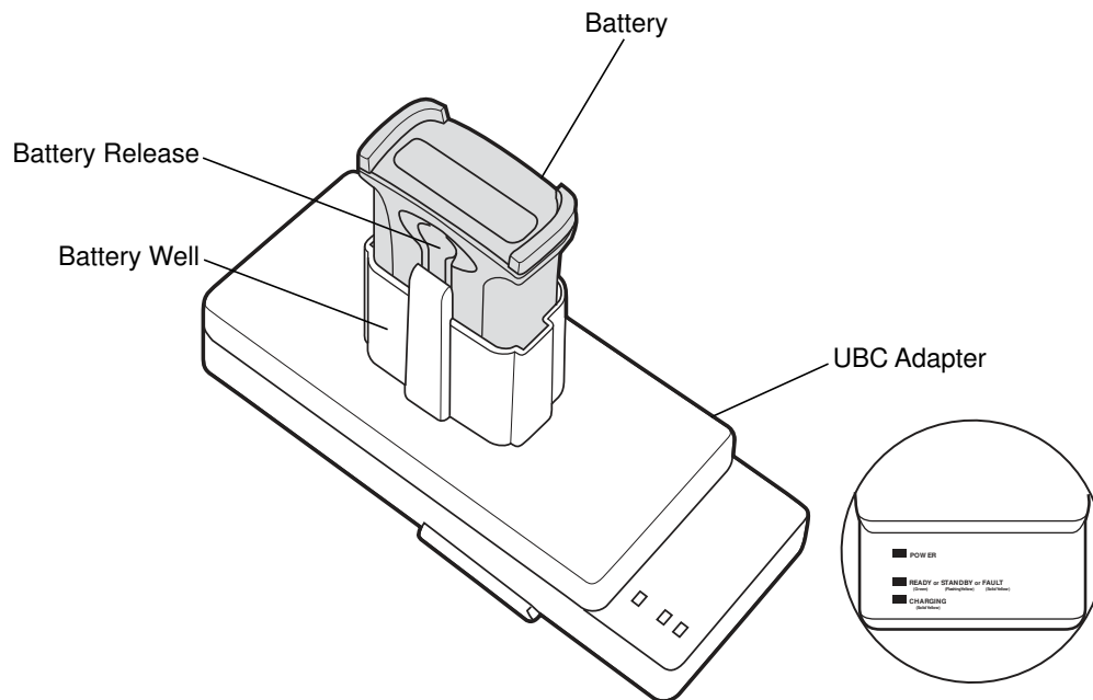
Figure 7-10 UBC Adapter
