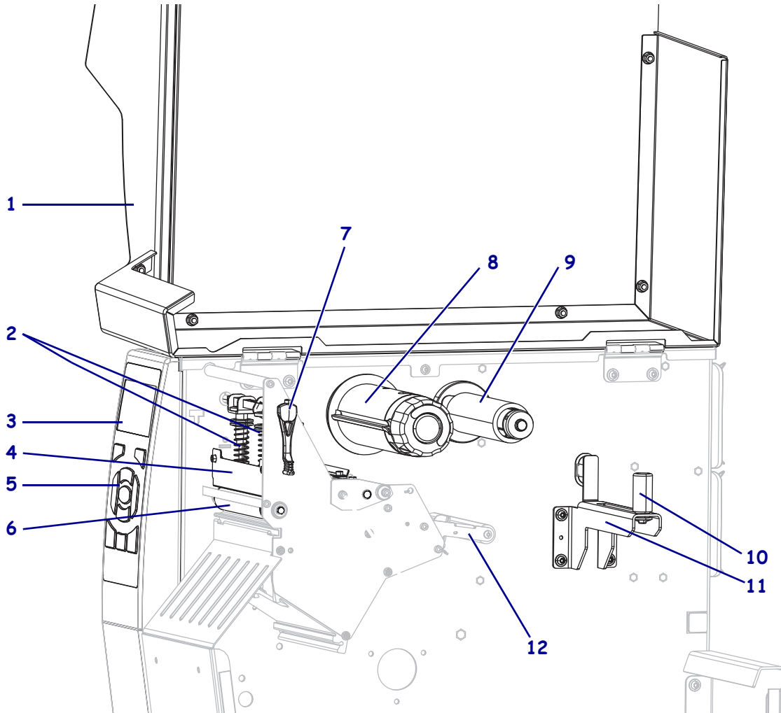
Figure 1 • Printer Components
