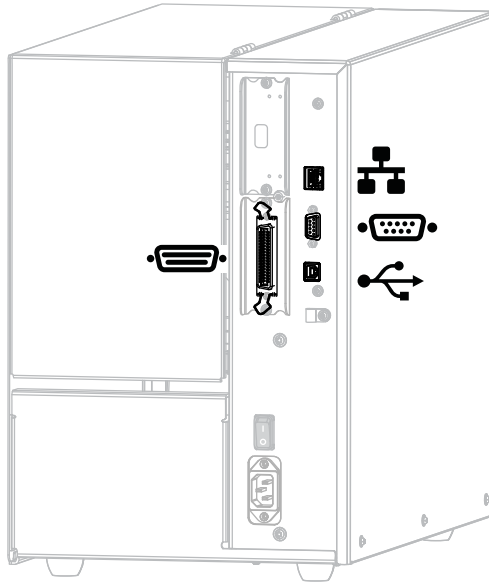
Figure 3 • Location of Communication Interfaces
