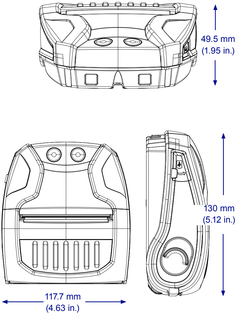
Figure 29 • ZQ320 Dimensions
