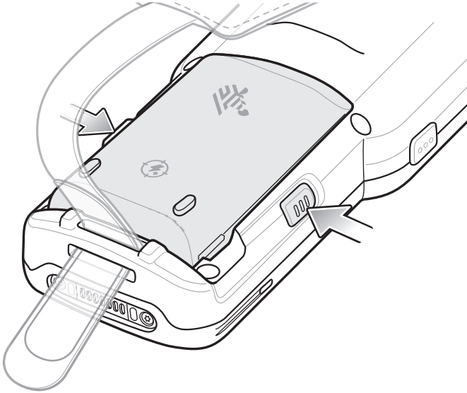
Figure 22 Release Battery
